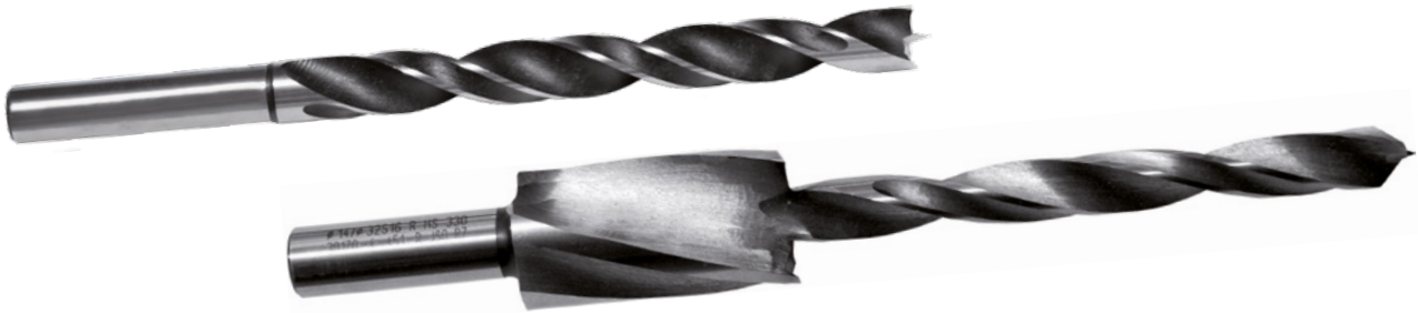
Drill for Speed-Cut Revolver mill
