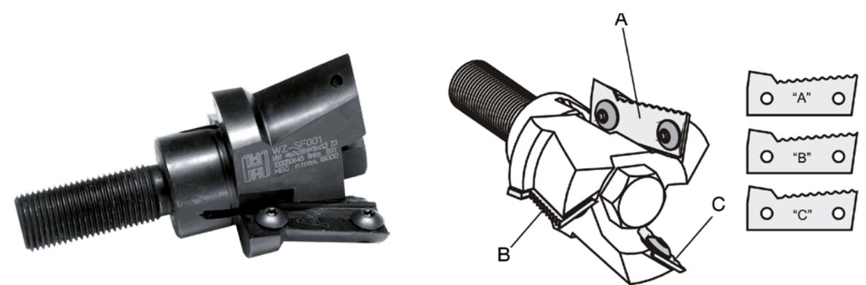
Dovetail milling cutters with replaceable cutters
